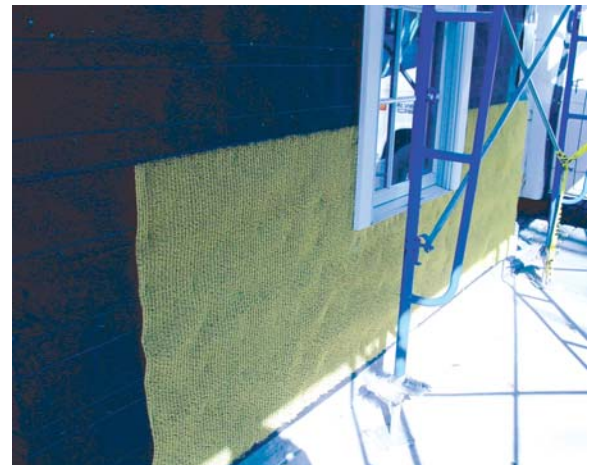
Photograph 8: Air Gap —The air gap does not have to be particularly big to be a big deal— 3/8 inch (9 mm). One method of getting the air gap is to use a drainage mat between two layers of building paper. The gap allows redistribution of the moisture in both the stucco and the OSB sheathing.
