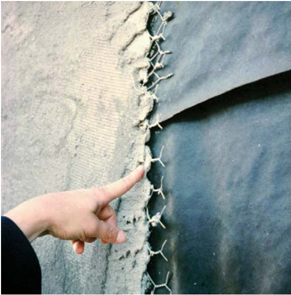
Photograph 2: Hardcoat Stucco —Three coats have been traditionally applied directly over a single layer of impregnated felt or asphalt saturated kraft paper. Today, this results in a bond between the stucco rendering and the outer layer of the felt or paper compromising drainage.
