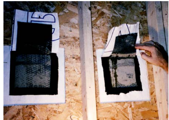
Photograph 7: Building Paper Bond Break —Traditional building paper is an excellent bond break between traditional hardcoat stucco and plastic building papers.
